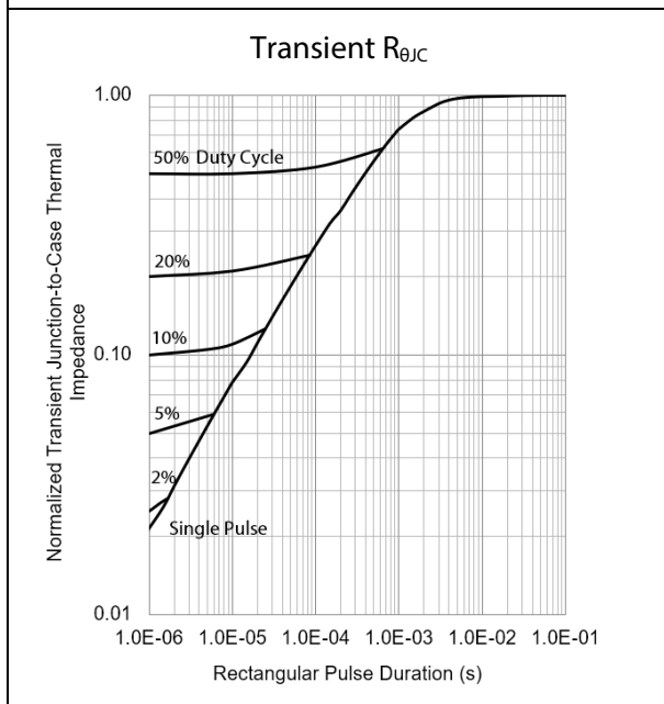
Figure 15: Transient Thermal Impedance 1.00 = Nominal DC thermal impedance
